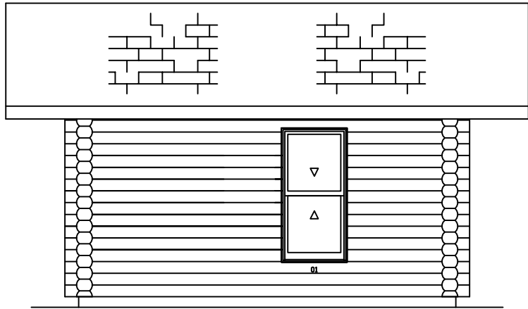
LEFT ELEVATION
