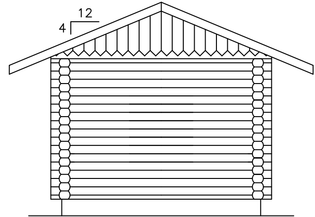
REAR ELEVATION
