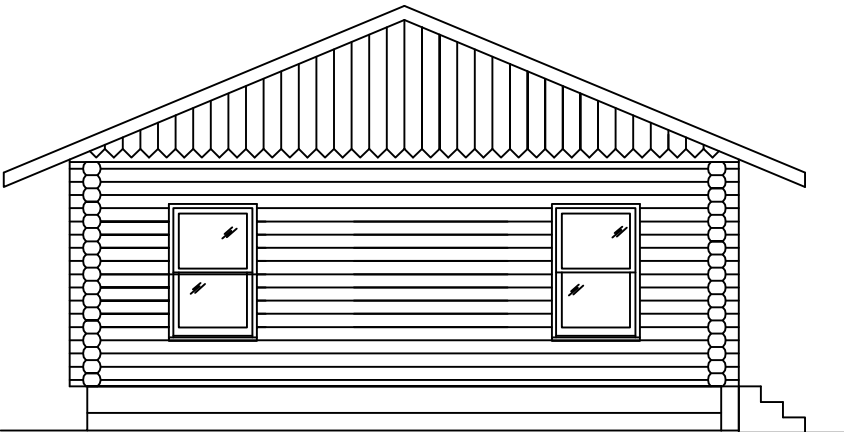
LEFT ELEVATION
