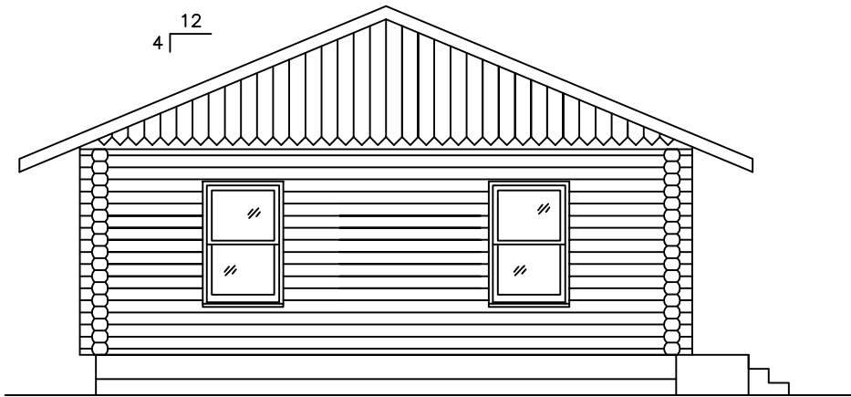
LEFT ELEVATION
