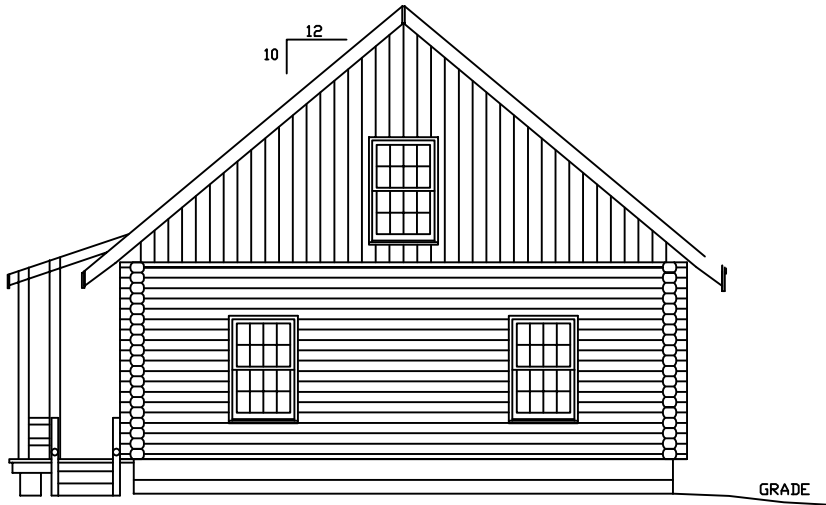
LEFT ELEVATION
